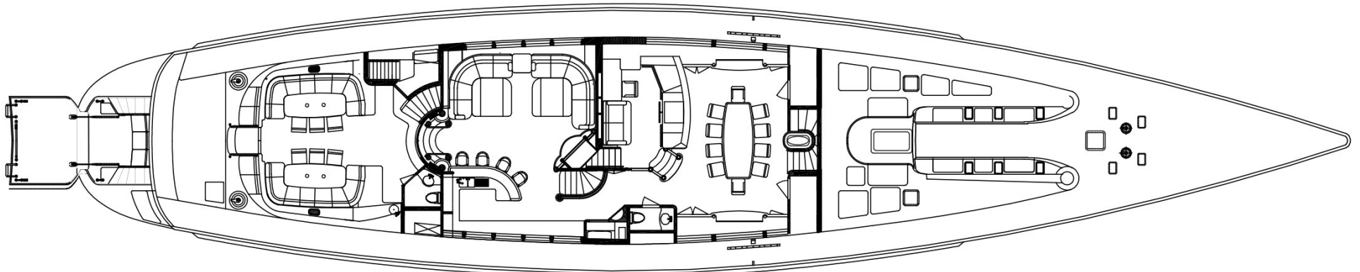
MAIN DECK PLAN
