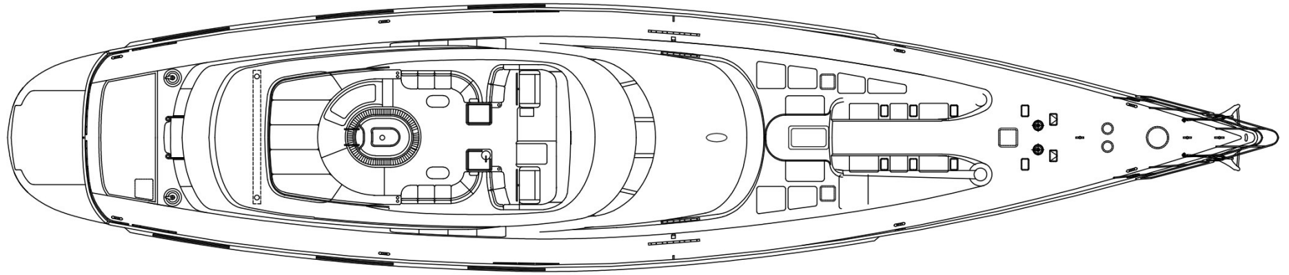
SUNDECK DECK PLAN
