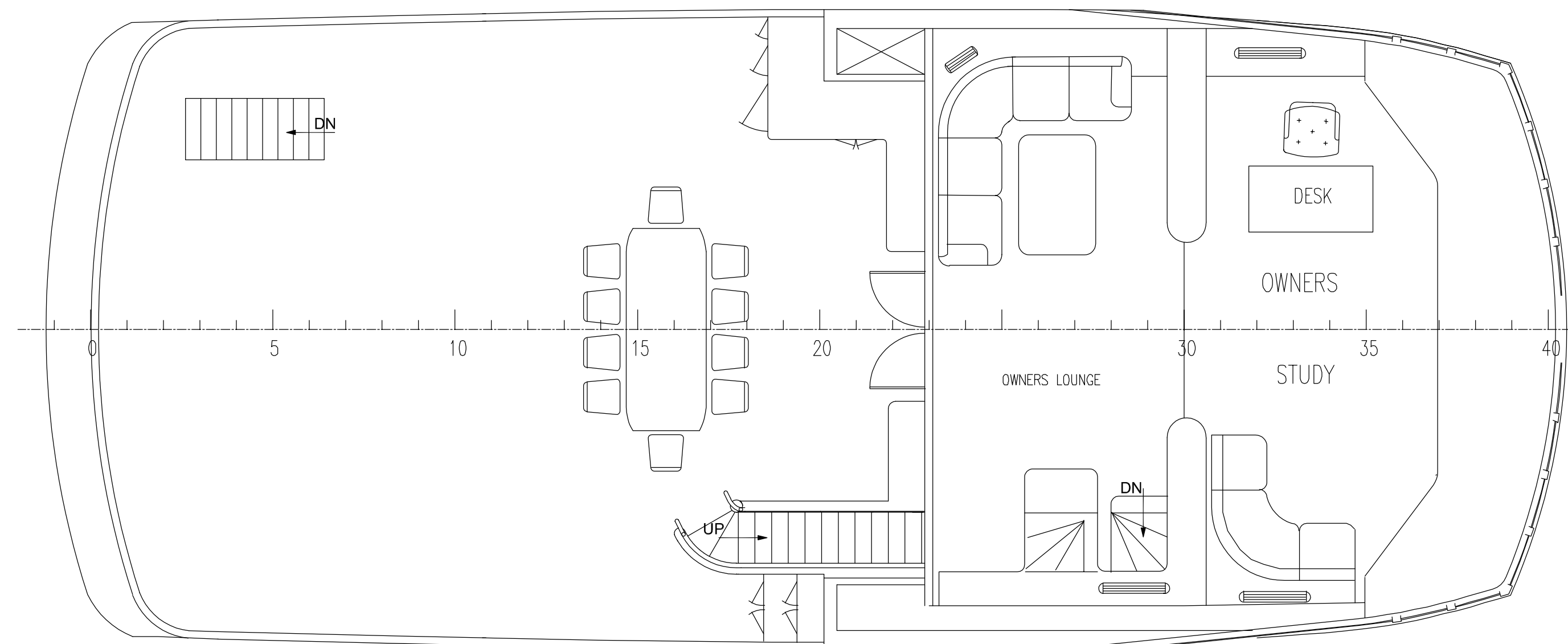
OWNER'S DECK
