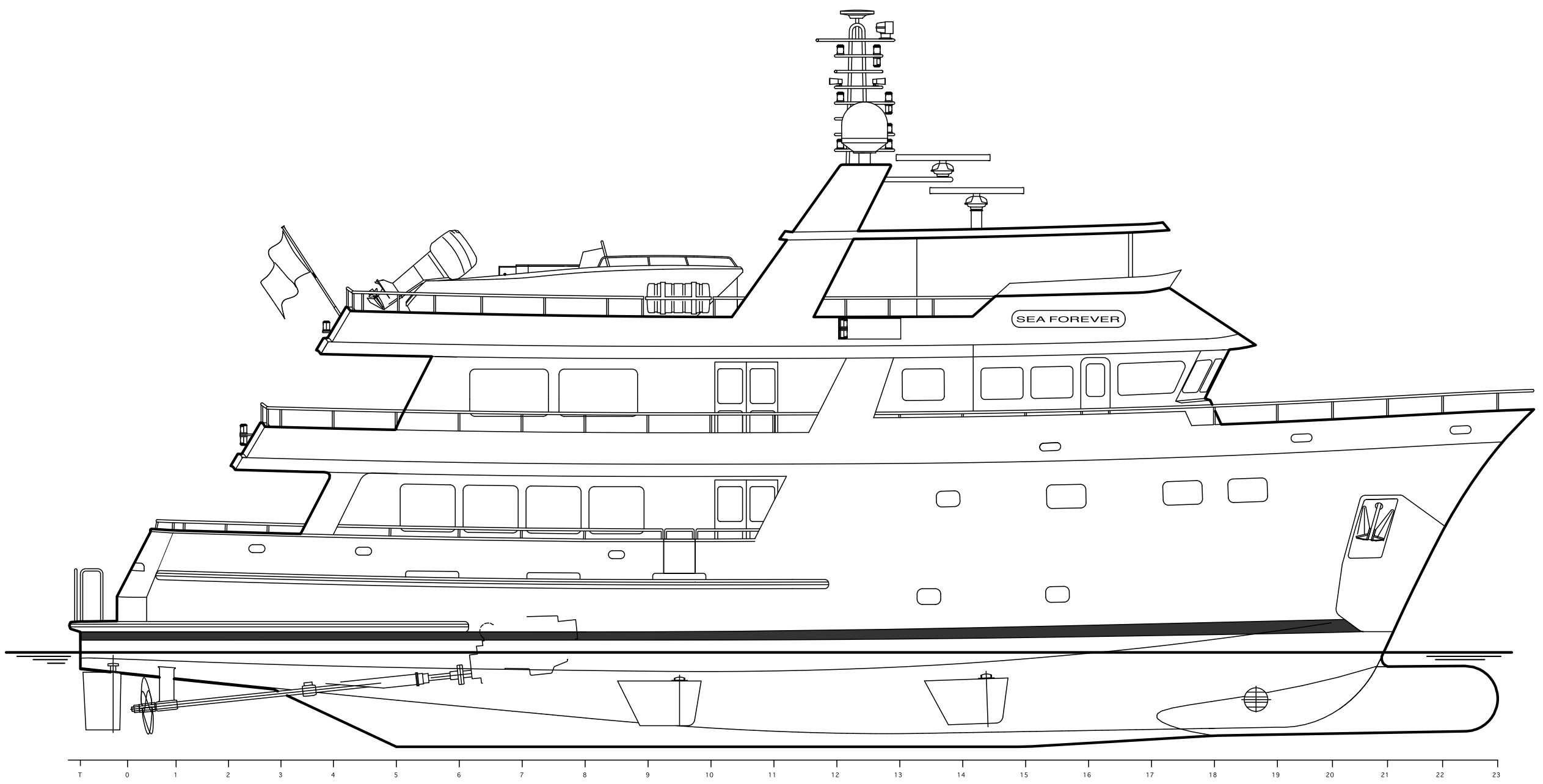
OUTBOARD PROFILE
